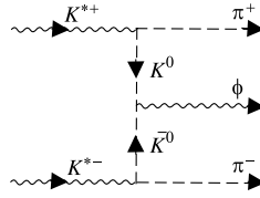
Fig. 10. Feynman diagram for the process K^{*+} K^{*-} \rightarrow \phi \pi^+ \pi^-
