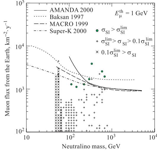
Fig. 12. High-energy muon flux predictions and experimental limits due to the annihilation of supersymmetric particles in the center of the earth. See Ref. 25 for explanation of symbols. The AMANDA limit (90 % C.L.) was corrected to correspond to a threshold of 1 GeV
