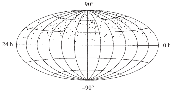
Fig. 4. Sky-plot in equatorial coordinates of the neutrino candidate events found by either of the two analyses
