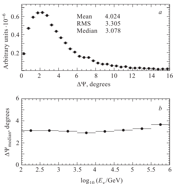
Fig. 5. Error in the space angle for simulated signal events with energy spectra proportional to E_{\nu}^{-2} : (a) distribution of error averaged over declination; (b) space angle error as a function of neutrino energy
