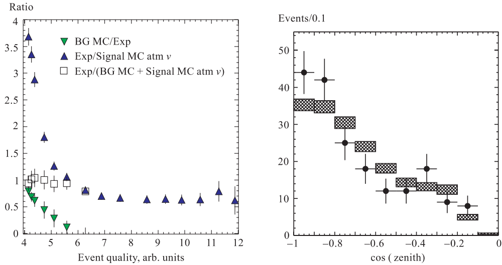
Fig. 2. Ratios of passing rates for simulated background (BG MC), simulated atmospheric neutrino signal (Signal MC atm \nu ), and reconstructed experimental data (Exp) as a function of «event quality», a variable which measures the severity of the selection criteria
