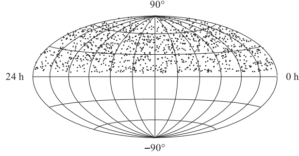
Fig. 6. Sky distribution of the 1097 events in the point source analysis. Coordinates are Right Ascension (RA) and declination (dec.). When looking for point sources, one does not optimize signal/noise. Instead, one is interested in \text{signal}/\sqrt{\text{noise}} for optimal significance. Thus the sample used in this analysis is about 6 times larger than that in the atmospheric neutrino analysis in Fig. 4
