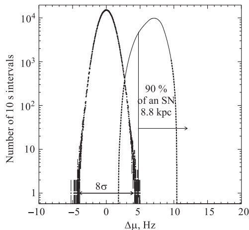
Fig. 11. 1997 & 1998 data (left distribution) compared to an equivalent data set simulated for SN1997-A type signals. 90 % of a Supernova neutrino burst located at 8.8 kpc distance would be seen above a cut for less than one fake event per year (vertical line)
