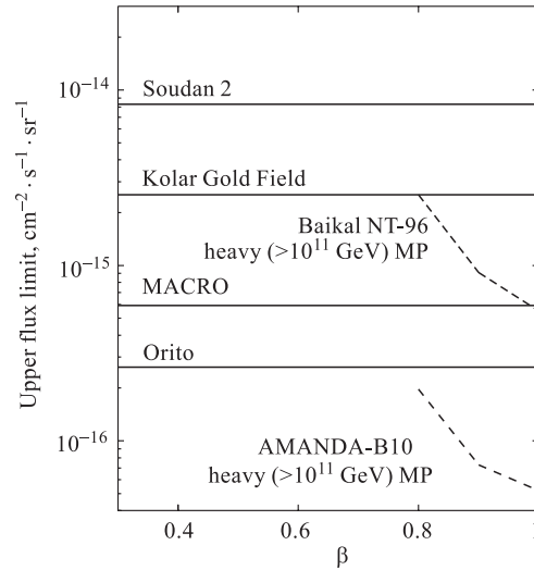
Fig. 13. Upper flux limit (90 % C.L.) for various experiments versus the monopole velocity. Taken from [32]
