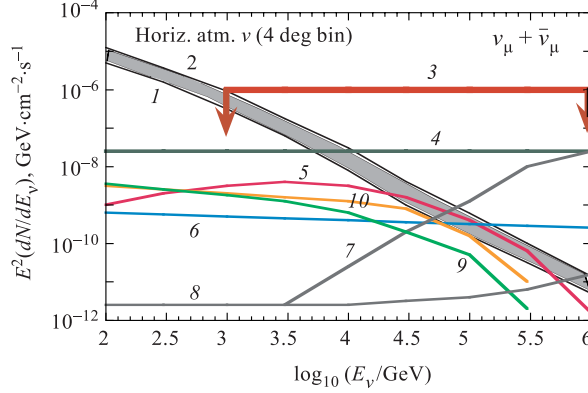
Fig. 1. Survey of \nu + \bar{\nu} flux predictions from cosmic accelerators of high-energy neutrinos (adopted from the recent review by Learned and Mannheim [6]). The atmospheric neutrino fluxes are from [7], for both vertical (1) and horizontal (2) fluxes within a circle defined by a half angle of 4 degrees (labeled «4 deg bin»). The curves do not include the normalization uncertainty, possibly 20% in magnitude. 3 — AMANDA-B10 limit reported here; 4 — Ref. 8 for the core emission from 3C273 due to pp interactions. It also represents neutrino emission from the AGN Blazar Mk501 during 1997 if it emits half of its TeV gamma ray flux in neutrinos; 5 — Crab Nebula, model I from [9]; 6 — Coma cluster according to [10]; 7 — core emission from 3C273 due to p-\gamma interactions [11]; 8 — model [12] for the relativistic jet of 3C273 including p-p and p-\gamma interactions, and Supernova remnant gamma-Cygni (9) and IC 444 (10) according to [13]. The energy bounds on the AMANDA limit are restricted to the approximate region of sensitivity of the detector
