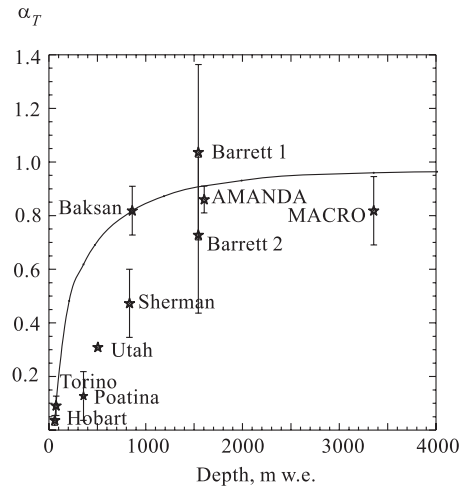
Fig. 14. Measurements of \alpha_T by detectors at different depths, with the expected curve and with AMANDA value added (From [35])
