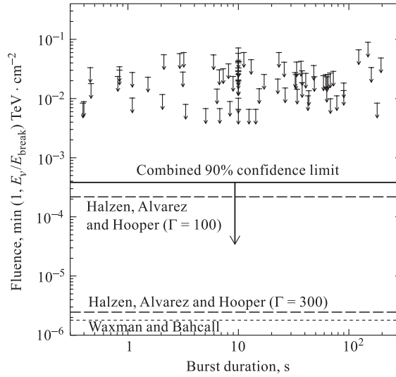
Fig. 10. Individual and combined limits on GRB fluence obtained from 78 GRBs. Theoretical predictions [19,22] are plotted for comparison
