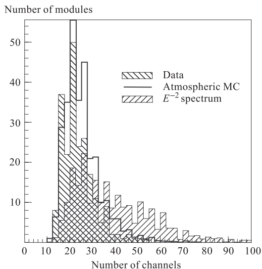
Fig. 9. Distribution of the number of optical modules for the data presented in Fig. 3. The MC simulations for atmospheric neutrinos and a generic spectrum 10^{-5} E^{-2} \text{cm}^{-2} \cdot \text{s}^{-1} \cdot \text{sr}^{-1} \cdot \text{GeV}^{-1} are also shown
