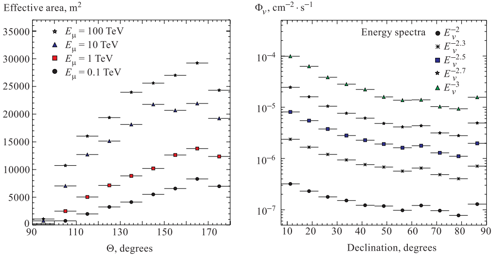
Fig. 7. The effective area for muon detection as a function of zenith angle for E_\mu between 0.1 and 100 TeV ( 180^\circ is vertically up in local detector coordinates)
