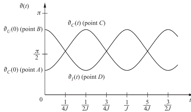
Fig. 6. Explicit variations of \vartheta_C(t) and \vartheta_I(t) angles showing oscillations as functions of time in the general case (formulae (68) and (73))
