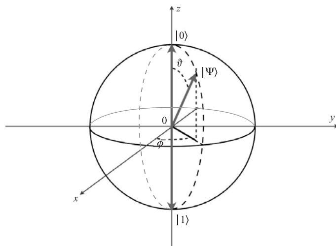
Fig. 1. Bloch's sphere which enables to represent the qubit |\Psi\rangle by a vector of polar angles \vartheta and \phi
