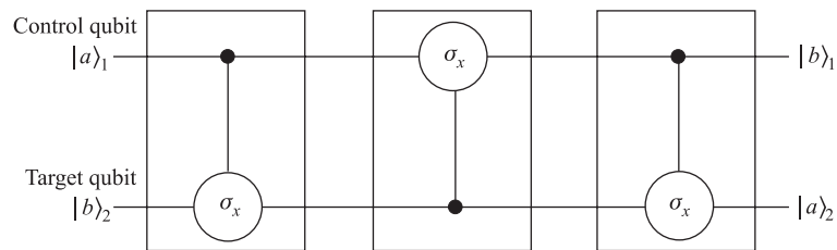
Fig. 4. Gate sequence \text{CNOT}_{12}\text{CNOT}_{21}\text{CNOT}_{12} giving a swapping
