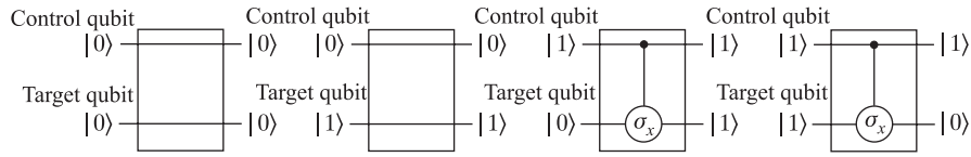
Fig. 2. Representation of the \text{CNOT}_{12} gate for base qubits (see formula (16))
