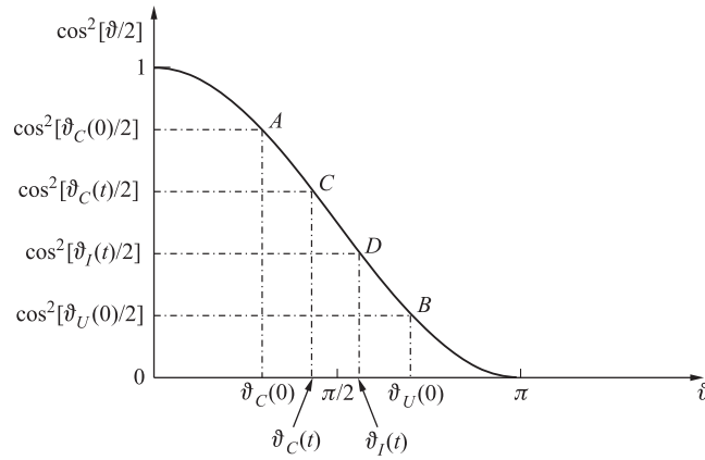
Fig. 5. Variations of \vartheta_C(t) and \vartheta_I(t) angles as functions of time in the general case (formulae (68) and (73))
