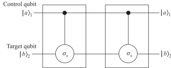
Fig. 3. Product of the \text{CNOT}_{12} gate by itself giving identity
