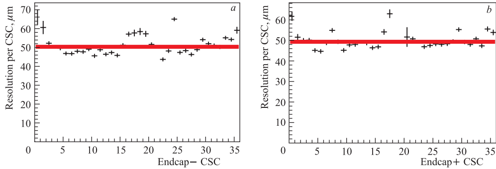
Fig. 8. ME1/1 outer part spatial resolution for both endcaps. The vertical bars show the statistical errors
