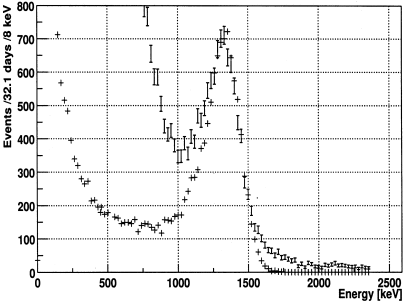
Figure 5: ^{40}\text{K} events in the CTF-II data (upper line) and MC simulation of the 1.46 MeV gamma (the lower one). The \beta -spectrum of the ^{40}\text{K} spectrum was not simulated. One can see the good agreement of the position of the peaks
