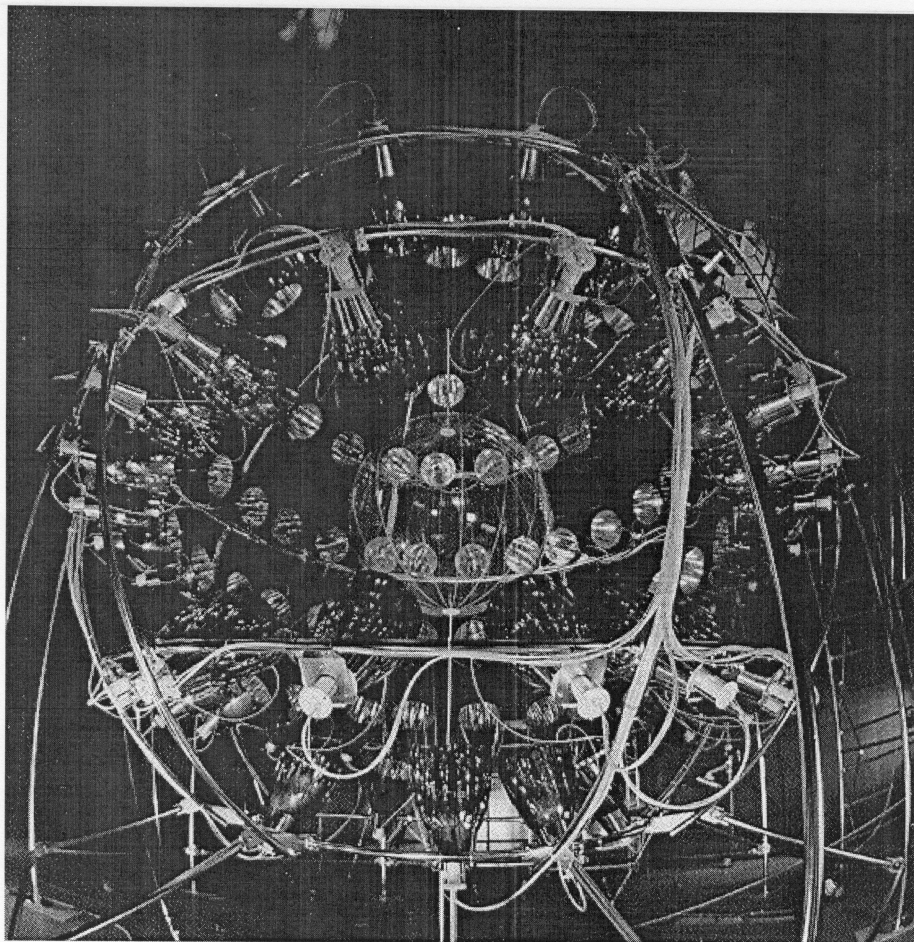
Figure 1: The view of the CTF detector
