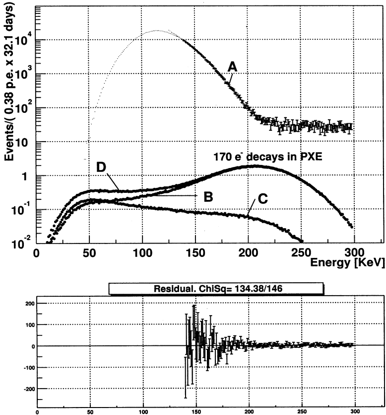
Figure 6: C^{14} spectrum (curve A) with superimposed fit curve and the results of 256 keV \gamma Monte-Carlo simulations. The Monte-Carlo results are normalized to 170 electron decay events in the inner vessel. An additional gammas, arriving from the decays in surrounding water are shown as well (curve C). The total detector's response to the 256 keV \gamma (curve D) is the sum of the gammas from PXE (curve B) and water surrounding the inner vessel with PXE (curve C). 0.38 p.e. bin correspond to 1.07 keV at the high energies.
