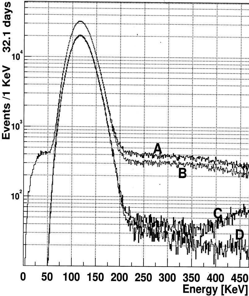
Figure 4: CTF-II background in the low energy region and the result of the sequential cuts applied in order to reduce background: A) raw data; B) muons cut; C) radial cut (with 100 cm radius); D) \alpha/\beta discrimination.
