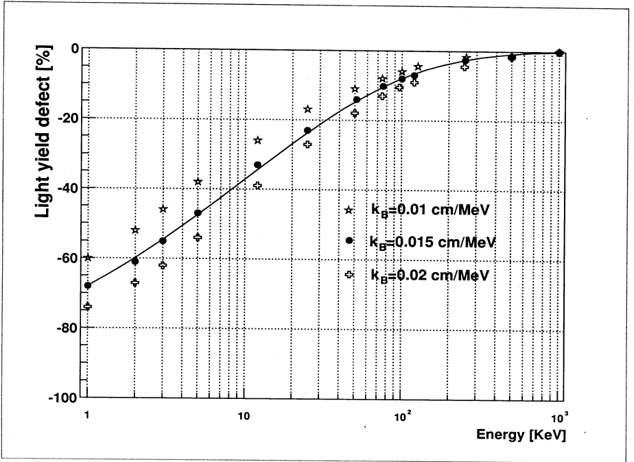
Figure 2: Light yield deficit for 3 different k_B values calculated for PC. The data for k_B = 0.015 cm/MeV are shown together with fit function (3)
