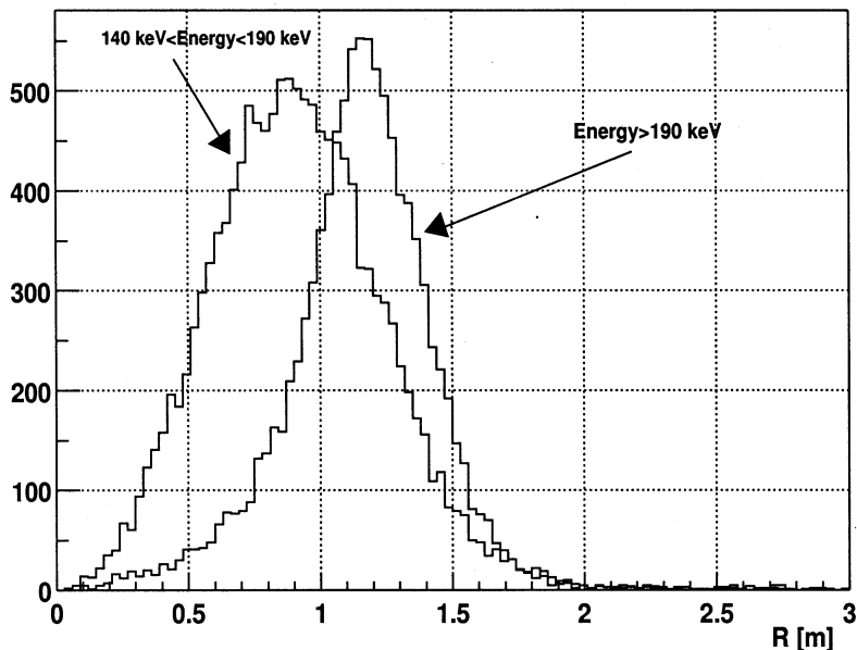
Figure 3: Radial distribution of the events in two different energy intervals. The events in the 140-190 keV interval are mainly ^{14}\text{C} events uniformly distributed over the detector's volume with the admixture of the external gammas. The major part of the events with energies greater than 190 keV are the caused by the decay of the ^{40}\text{K} , located mainly near the detectors surface.
