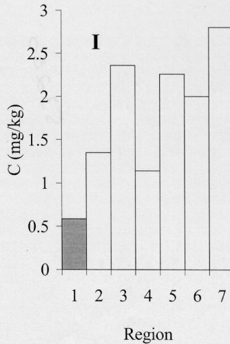
Fig. 2. Comparison of present results with concentration levels in moss from selected sites in Europe investigated by the authors: 1 - Baia Mare; 2 - Karabash, South Ural Mountains (copper smelter); 3 - Tula, central Russia (mixed industry); 4 - «Copper Basin», Poland; 5 - Mo, northern Norway (ferro-alloy smelters); 6 - Median value, Norway 2000.
