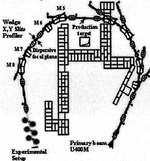
Fig. 2. Schematic diagram of the beam-line for producing the secondary beam with the position of the present setup.
