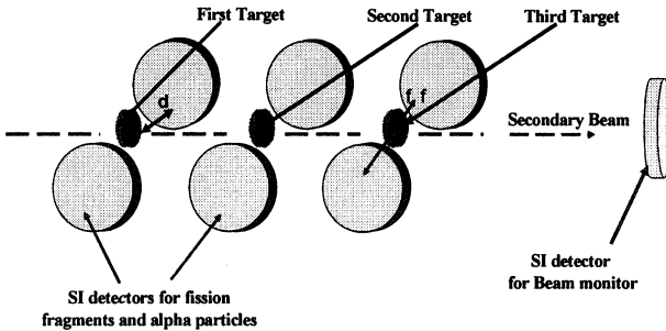
Fig. 1. Layout of the experimental setup.
