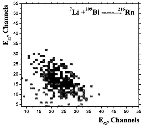
Fig. 4. The two-dimensional plot of the energies of the two correlated fission fragments obtained in the {}^7\text{Li}+{}^{209}\text{Bi} -reaction.
