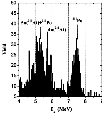
Fig. 5. Experimental \alpha -particle energy spectrum, measured after the emission of different number of neutrons from the compound nucleus {}^{215}\text{At} .
