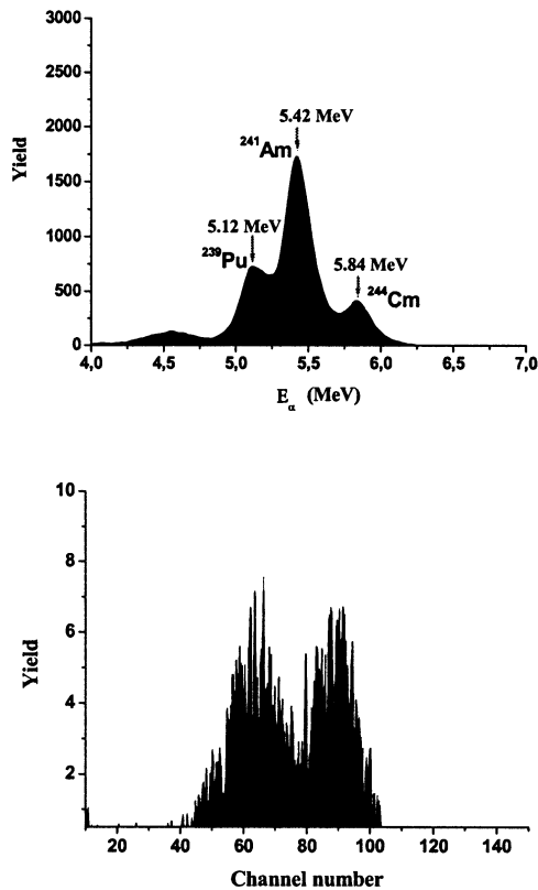
Fig. 3. Energy spectrum of \alpha -particles emitted by a Pu-Am-Cm source (upper panel) and energy distribution of fission fragments from the spontaneous fission of ^{244}\text{Cm} (lower panel).
