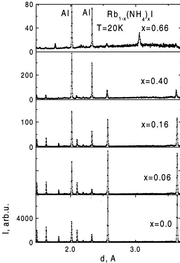
Fig. 1. The NPD spectra of Rb_{1-x}(NH_4)_xI ( x=0.0 ; 0.06 ; 0.16 ; 0.40 ; 0.66 ) mixed crystals obtained with the NERA-PR spectrometer.
