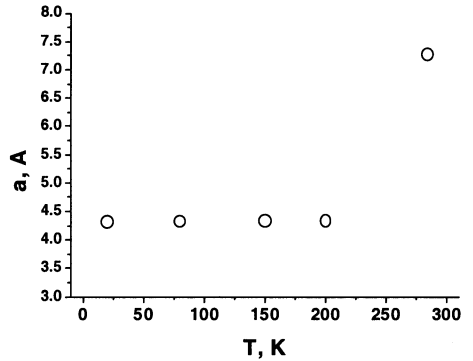
Fig.3 (c). The lattice parameter a of the cubic structure of Rb_{0.23}(NH_4)_{0.77}I mixed crystals as a function of temperature.
