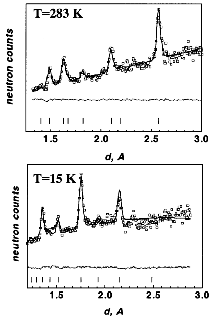
Fig. 2 (b). The diffraction patterns of \text{Rb}_{0.23}(\text{NH}_4)_{0.77}\text{I} at 283 K (sp.gr. Fm\bar{3}m ) and 15 K (sp.gr. Pm\bar{3}m )
