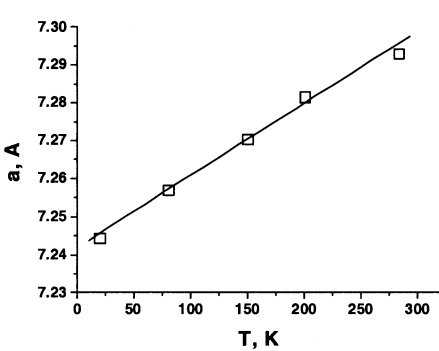
Fig. 3 (b). The lattice parameter a of the cubic structure of Rb_{0.71}(NH_4)_{0.29}I mixed crystals as a function of temperature.
