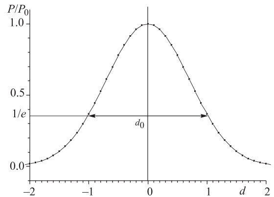
Fig. 5. Power density distribution in the one-mode laser ray cross section
