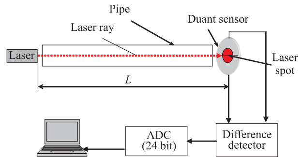
Fig. 14. Experimental setup
