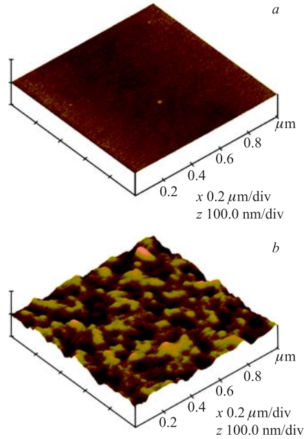
Fig. 2. Three-dimensional projected AFM images of 1 \times 1 \mu\text{m} scanned areas of (a) unirradiated InP and (b) 1 \cdot 10^{14} ions/cm 2 irradiated InP surface. Vertical scale = 100 nm/div
