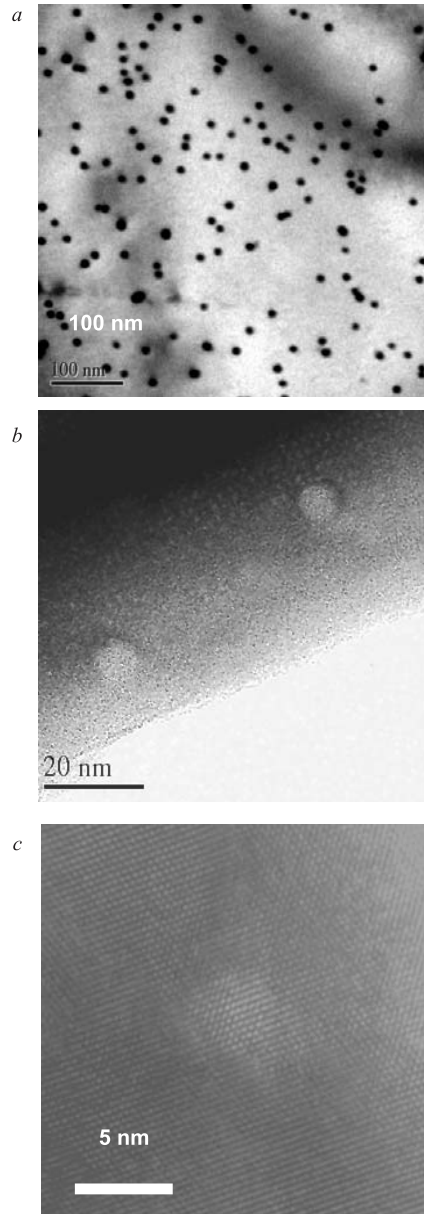
Fig. 5. Bulk ion tracks observed by TEM in InP: (a) a field of ion tracks; (b) a high magnification TEM of two tracks; (c) HRTEM of a single ion track
