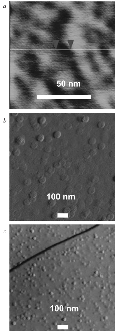
Fig. 4. The AFM image of 100 \times 100 nm scanned area of InP irradiated with fluence of 5 \cdot 10^{10} ions/cm 2 showing a pit-like feature identified with surface-ion tracks due to single 200 MeV Au + ion impact, the width of the pit \sim 12.5 nm. In (b) and (c) AFM images of 1 \times 1 \mu\text{m} scanned area of both muscovite mica and molybdenum disulphide respectively irradiated to the same ion fluence depicting the observed prominent surface-ion tracks are shown
