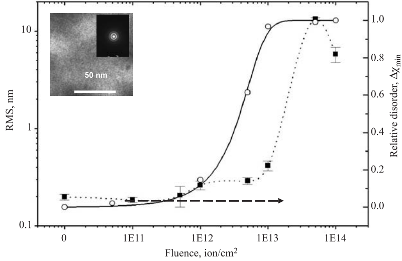
Fig. 7. The RMS roughness (nm) as a function of 200 MeV \text{Au}^+ ion fluence in InP (dotted line). The relative disorder induced by irradiation (solid line) is also plotted. The inset is TEM micrograph of InP irradiated to fluence of 5 \cdot 10^{13} ions/cm 2 , where the selected area diffraction pattern shows the diffused rings synonymous with amorphous material
