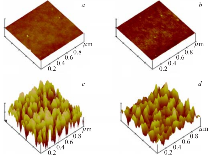
Fig. 6. Three-dimensional projected AFM images of 1 \times 1 \mu\text{m} scanned areas of (a) unirradiated surface, (b) 1 \cdot 10^{11} , (c) 5 \cdot 10^{13} and (d) 1 \cdot 10^{14} ions/cm 2 irradiated (001) InP surfaces. The surfaces for lower fluence irradiations are smooth on that scale (the height scale for all scans is 20 nm/division). The significant increase in surface roughness only occurs for higher fluences when the surface becomes completely amorphous. The observed surface modification in the form of hillock-like features is evident for the two highest ion fluences
