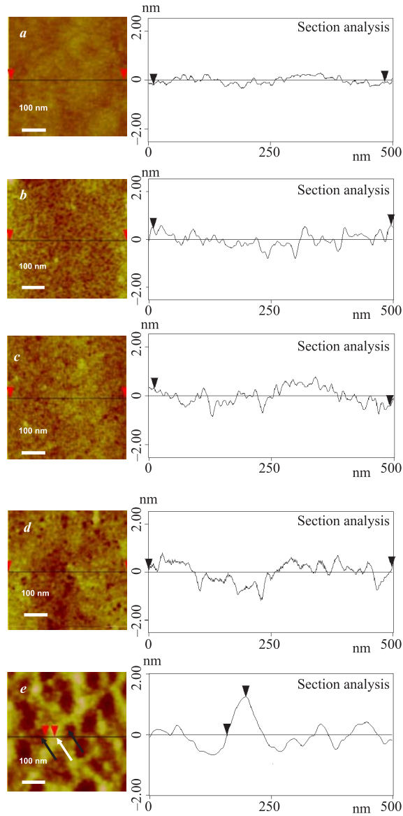
Fig. 1. The AFM images of 500 \times 500 nm scanned areas and sectional analyses across the surface of (a) unirradiated InP for (b) 5 \cdot 10^{10} ions/cm 2 , (c) 5 \cdot 10^{12} ions/cm 2 , (d) 1 \cdot 10^{13} ions/cm 2 and (e) 1 \cdot 10^{14} ions/cm 2 irradiated InP
