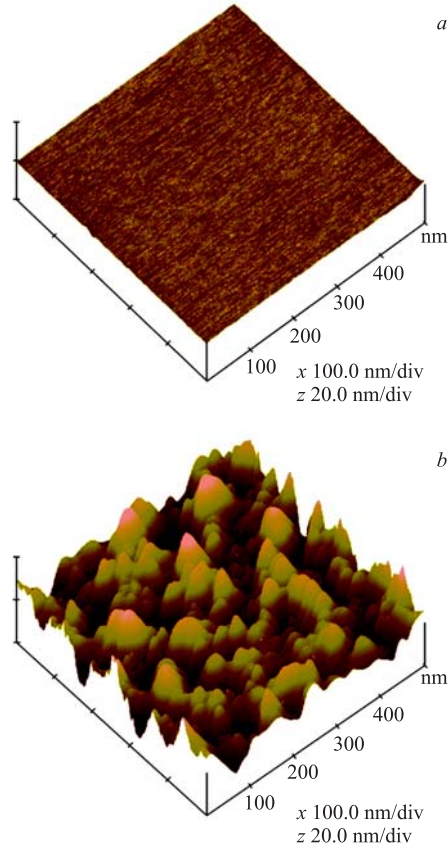
Fig. 3. Three-dimensional projected AFM images of 500 \times 500 nm scanned areas of (a) an area unexposed to the ion beam for the 1 \cdot 10^{14} ions/cm 2 irradiated InP sample (i.e., still crystalline) and (b) irradiated area of the same sample (amorphous). Vertical scale = 20 nm/div
