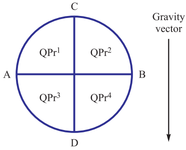
Fig. 9. Position of the quadrant photodetector for horizontally (A, B) and vertically (C, D) performed measurements
