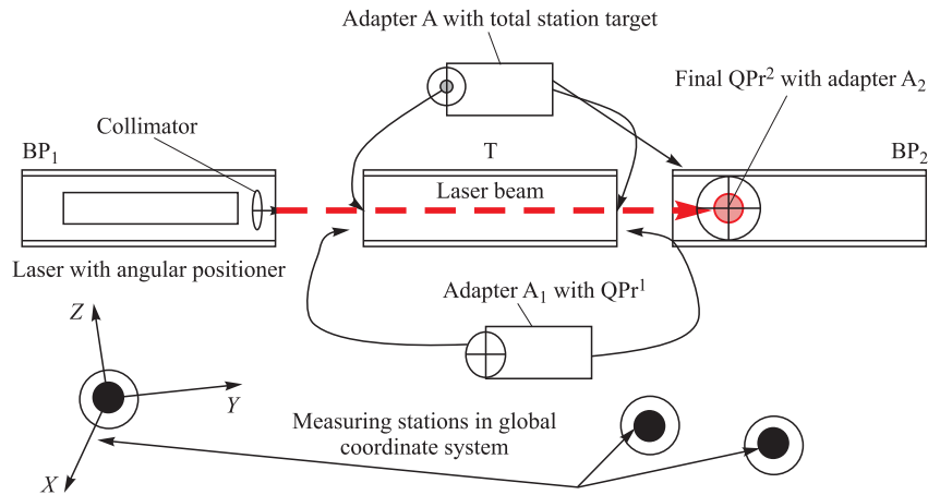
Fig. 3. The LRL measurement system for precise measurement of two transverse coordinates of the beam-pipe mock-up T
