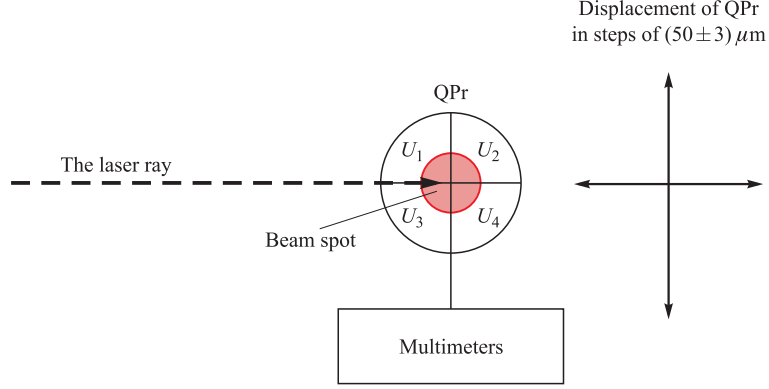
Fig. 8. Diagram of calibration measurements with a single-mode laser beam
