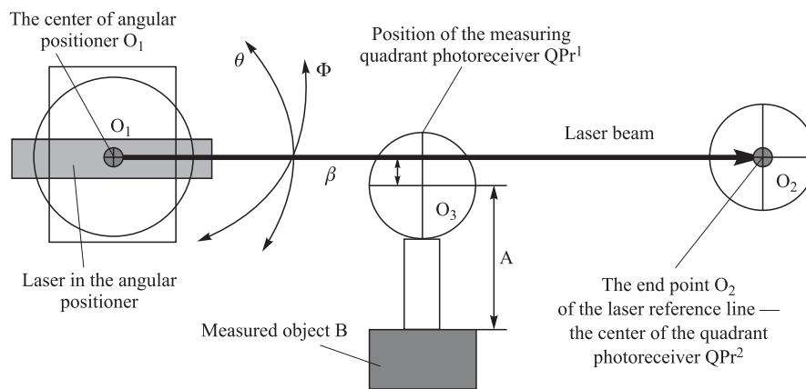
Fig. 2. Diagram of the LRL system
