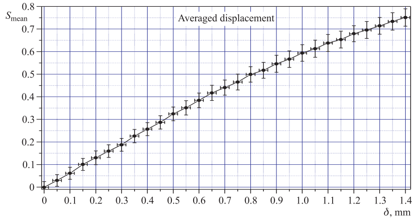
Fig. 15. Averaged calibration values S_{\text{mean}} as a function of \delta
