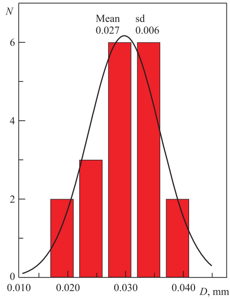
Fig. 14. Distribution of D = \bar{S}_{\text{hor}} - \bar{S}_{\text{vert}} as obtained from the calibration plots
