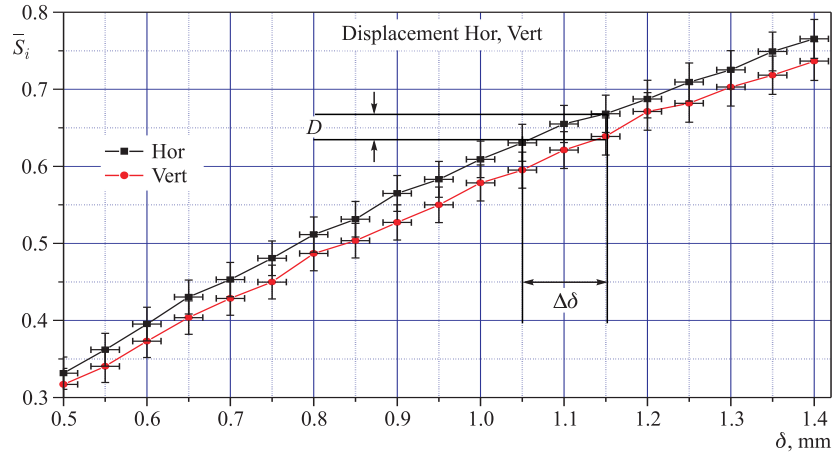
Fig. 13. Dependence of \bar{S}_{\text{hor}} and \bar{S}_{\text{vert}} on the displacement \delta when \delta \geq 0.5 mm
