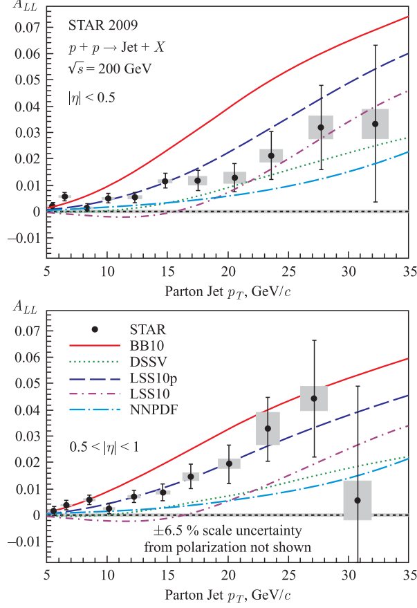
Fig. 2. Double longitudinal spin asymmetry of jet production in \vec{p} + \vec{p} collisions at \sqrt{s} = 200 GeV, |\eta| < 0.5 and 0.5 < |\eta| < 1 measured by the STAR Collaboration at RHIC [3]
