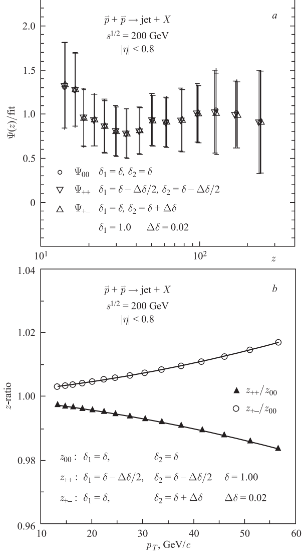
Fig. 3. a) The scaled spin-dependent \Psi_{++} , \Psi_{+-} and spin-independent \Psi_{00} functions for the process \bar{p} + \bar{p} \rightarrow \text{jet} + X at \sqrt{s} = 200 GeV and |\eta| < 0.8 in z -presentation. b) The ratios of the spin-dependent self-similarity parameters
