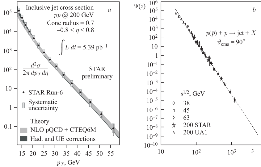
Fig. 1. a ) Inclusive spectra of jet production in p + p collisions at \sqrt{s} = 200 GeV and |\eta| < 0.8 measured by the STAR Collaboration [24] at RHIC. b ) The same data in z -presentation. The ISR and Sp\bar{p}S data from the analysis [17, 18] are shown for comparison
