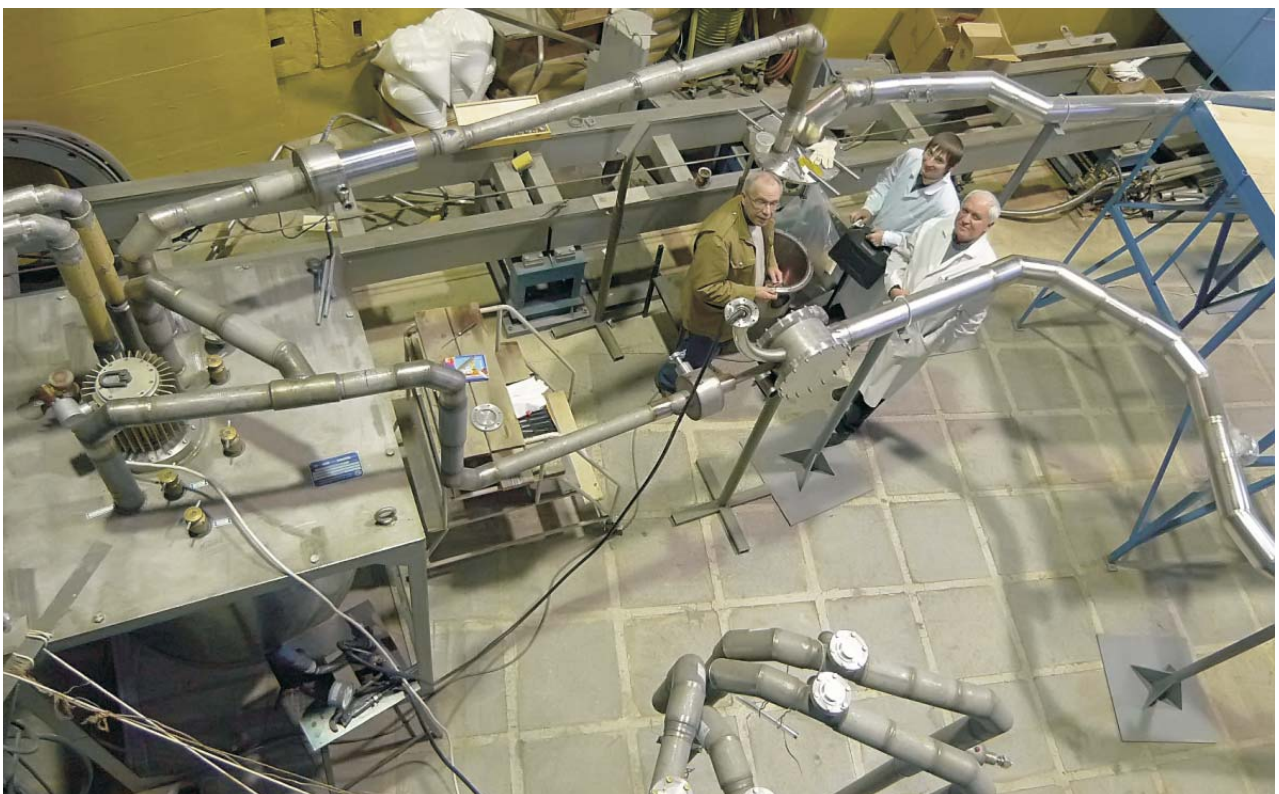
Frank Laboratory of Neutron Physics. Full-scale test bench for testing of the new cryogenic moderator of the IBR-2M reactor
